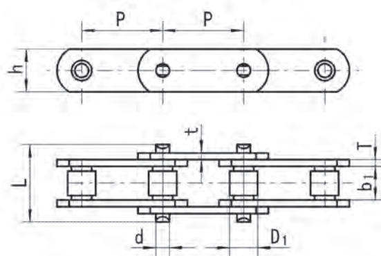
“S” roller type
