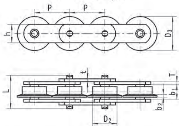
“F” roller type
