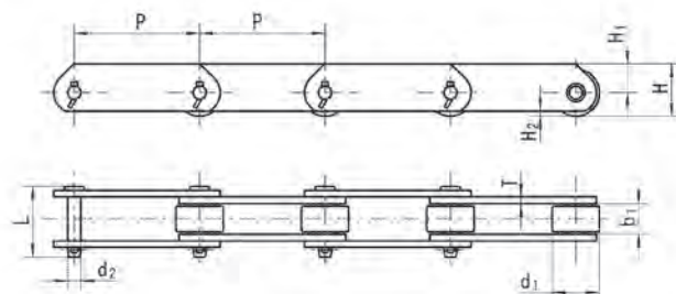
HA型附件 HA ATTACHMENT
