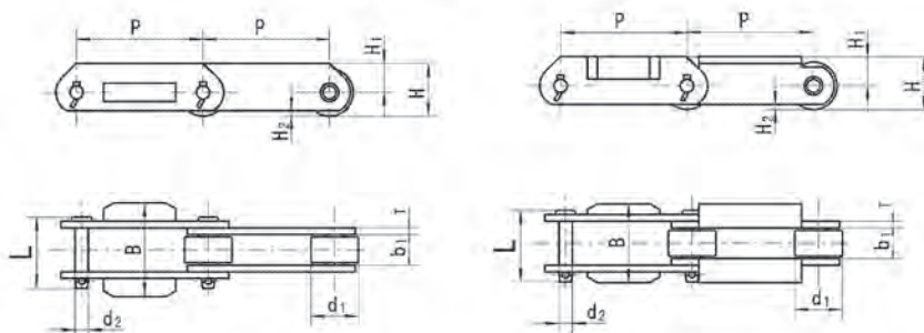
HB型附件 HA ATTACHMENT
