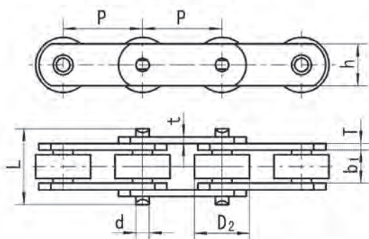
“R” roller type
